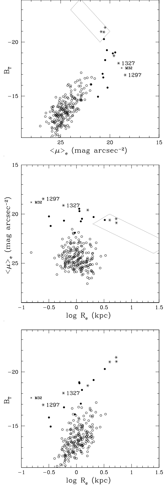
Fig. 10. Correlations among structural parameters of dE-E galaxies in the Virgo cluster. B_T vs. \langle \mu \rangle_e (top); \langle \mu \rangle_e vs. \log R_e (middle); B_T vs. \log R_e (bottom). The position of M32 (scaled to the distance of Virgo and corrected for B-V=1) as given by Faber et al. (1997) is marked with a cross. The dotted rectangle represents the loci of luminous "core" galaxies adapted from GG03.
