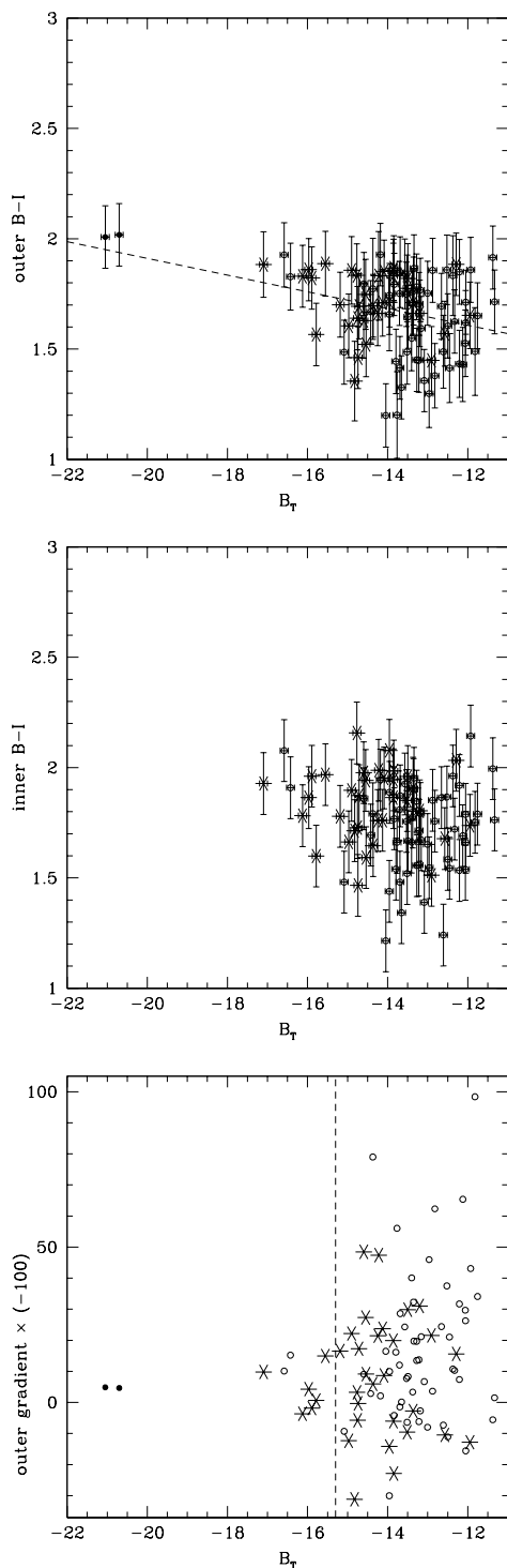
Fig. 8. The outer B-I color index (top); the inner B-I color index (middle; the two brightest objects are missing in this panel because they are both saturated) and the outer B-I gradient (bottom) as a function of B_T . In this figure filled dots represent giant Es, empty dots dEs, asterisks Nucleated dEs.
