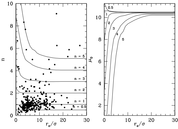
Fig. 4. The effect of the seeing on n (left) and on \mu_0 (right) as derived from the simulations (lines) for various n . Dots give the distribution of the observed points in the n - r_e/\sigma plane.
