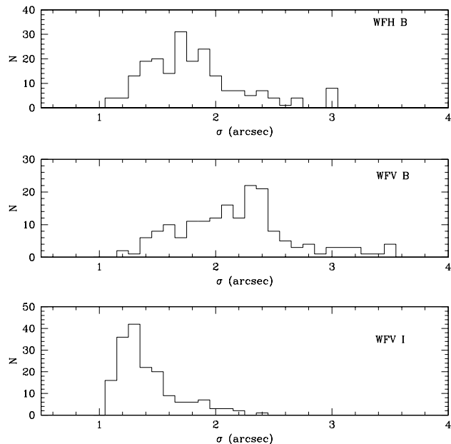
Fig. 3. Distribution of the seeing in the WFS.
