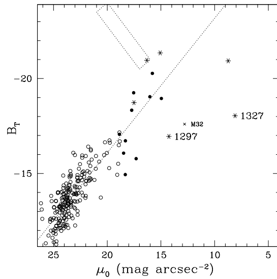
Fig. 11. Correlation between B_T and \mu_o for dE-E galaxies in the Virgo cluster. The position of M32 is marked with a cross. The dotted rectangle represents the loci of luminous "core" galaxies adapted from GG03. The dashed line gives the bisector linear regression.
