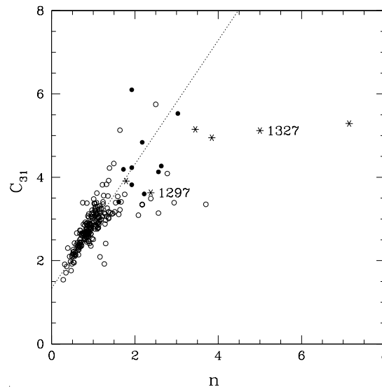
Fig. 12. Distribution of C_{31} versus n . The dashed line gives the bisector linear regression: C_{31} = 1.49 \times n + 1.33
